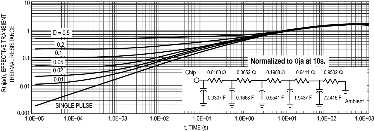
Figure 14. Thermal Response
