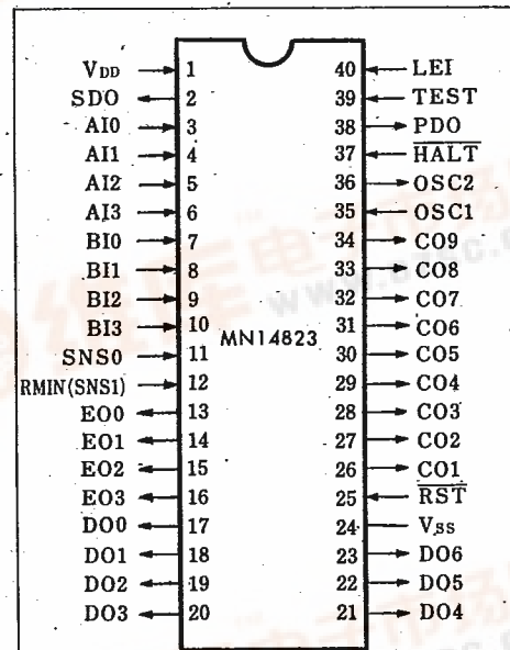
② 40-SDIP
