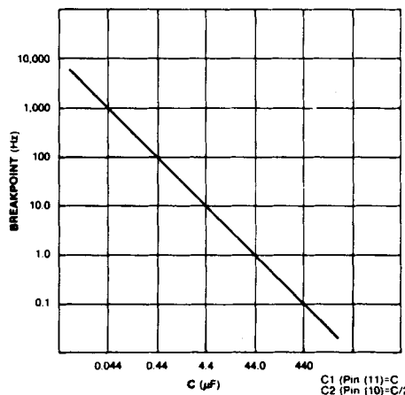
FILTER BREAKPOINT
