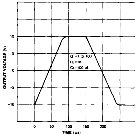
STEP RESPONSE
