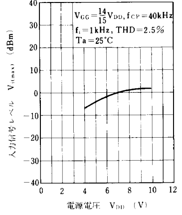
V_{i(max.)} - V_{DD}
