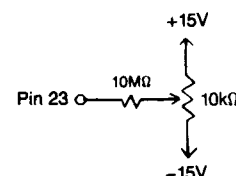
GAIN ADJUST
