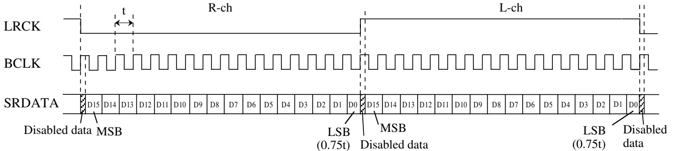
Figure 7-2-3 LRCK, BCLK and SRDATA output timing with de-emphasis function ON
