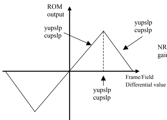
Fig. 3.6-2 NR-ROM characteristics
