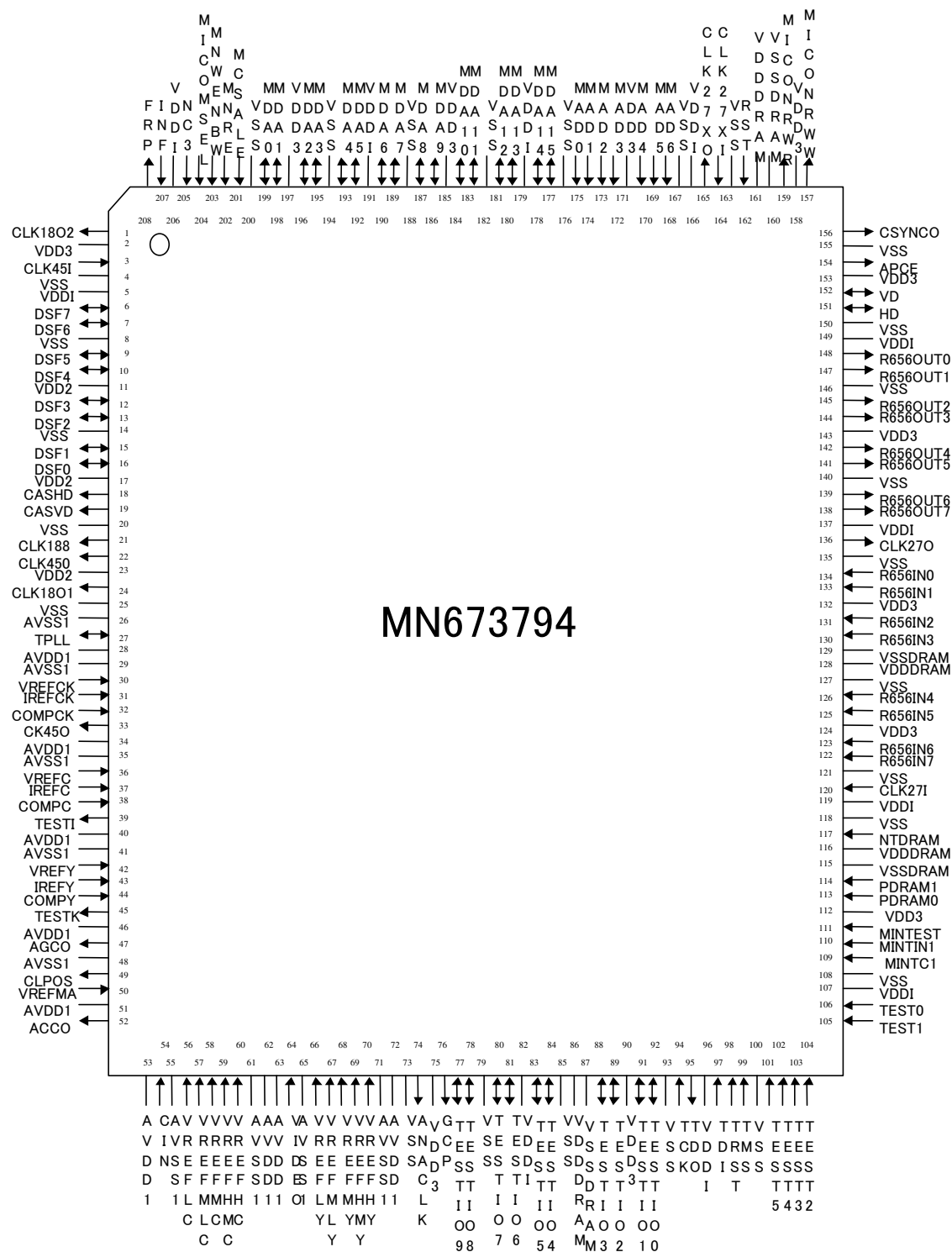
Figure 2.3 Pin Assignment
