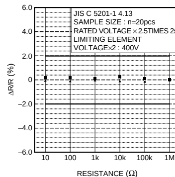
Fig.4 Overload
