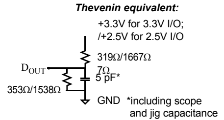
Figure C: Output load(B)
