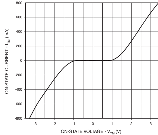
Figure 2 On-State Characteristics
