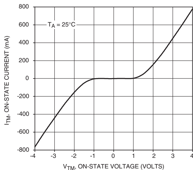
Figure 6. On-State Characteristics
