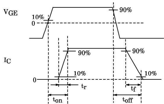
Waveform
