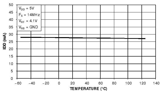
Figure 15. IDD vs TEMPERATURE
