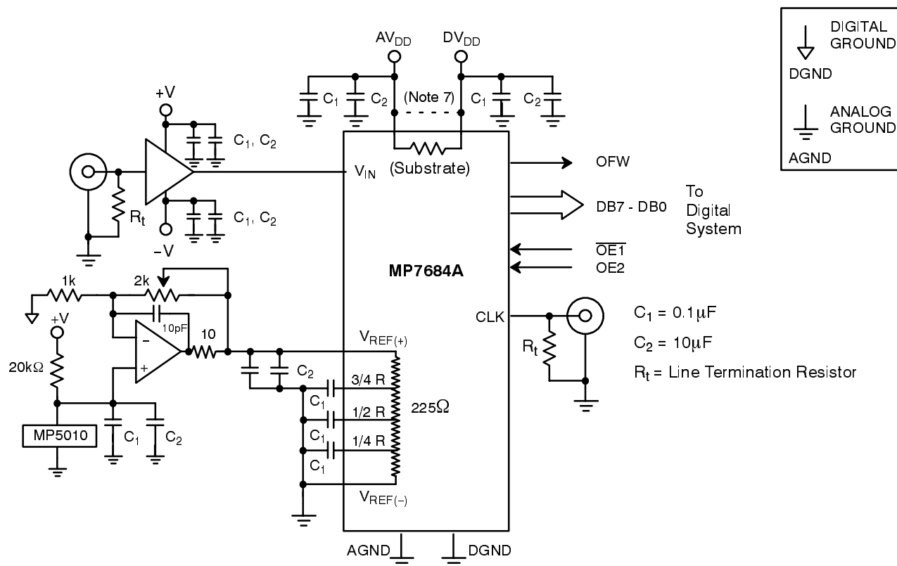
Figure 22. Typical Circuit Connections
