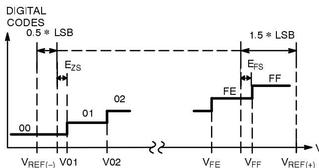
Figure 19. Real A/D Transfer Curve
