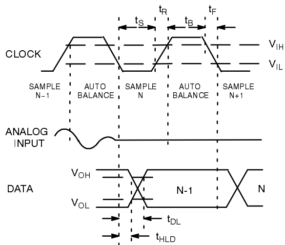
Figure 1. MP7684A Timing Diagram
