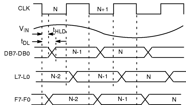
Figure 21. MP7684A Functional Equivalent Circuit and Interface Timing
