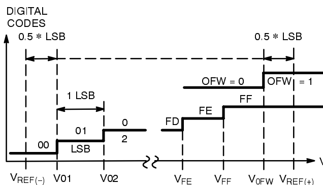
Figure 18. Ideal A/D Transfer Function
