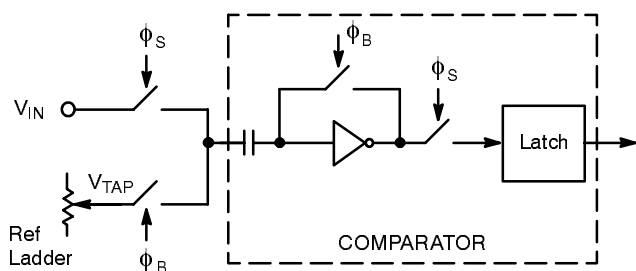
Figure 17. MP7684A Comparator
