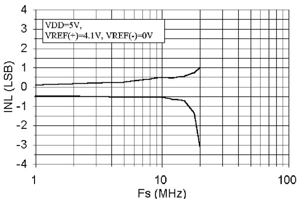
Figure 24. INL vs. Sampling Frequency
