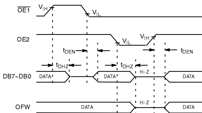
Figure 2. Output Enable/Disable Timing Diagram
