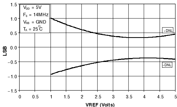
Figure 12. DNL vs VREF
