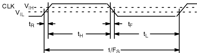
Figure 1. Clock Timing Specification
