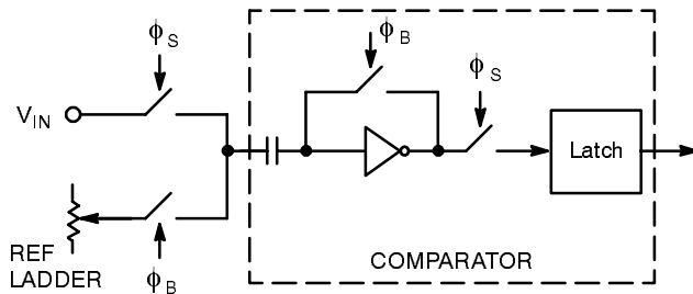
Figure 10. MP7686 Comparator
