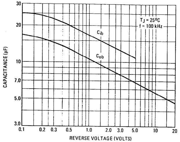
FIGURE 9 – CAPACITANCE
