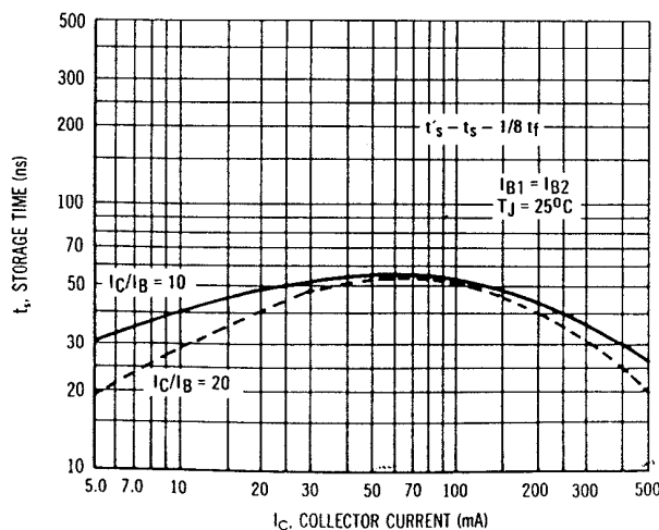
FIGURE 22 – STORAGE TIME
