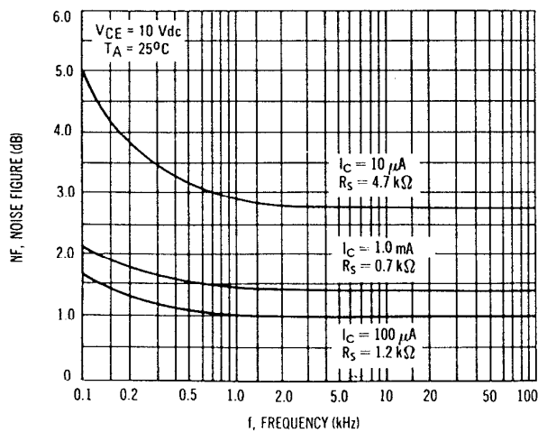
FIGURE 16 – FREQUENCY EFFECTS
