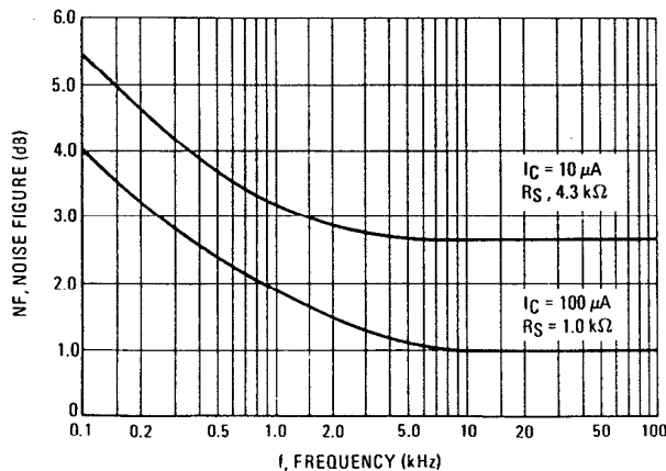
FIGURE 6 – FREQUENCY EFFECTS
