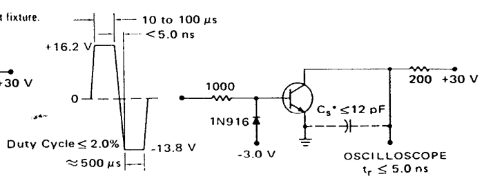
FIGURE 2 - NPN TURN-OFF TIME
