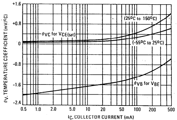
FIGURE 5 – TEMPERATURE COEFFICIENTS
