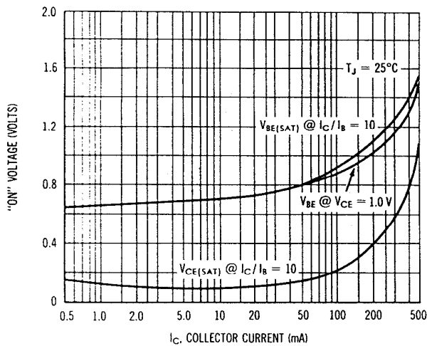
FIGURE 14 – "ON" VOLTAGES
