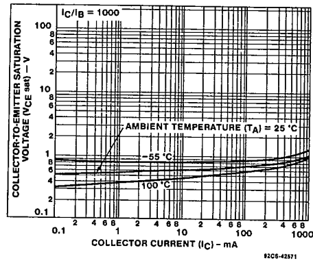
Fig. 2 - Typical collector-to-emitter saturation voltage characteristics.
