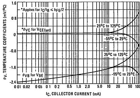
FIGURE 4 - TEMPERATURE COEFFICIENTS
