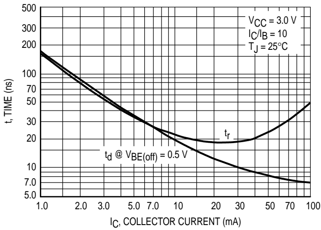
Figure 11. Turn-On Time
