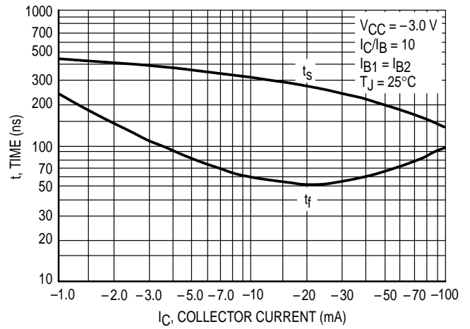
Figure 12. Turn-Off Time
