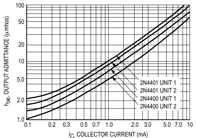
Figure 14. Output Admittance
