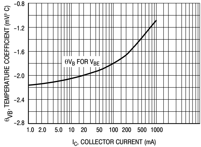
Figure 4. Temperature Coefficient
