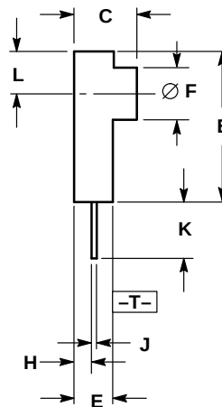
END VIEW
