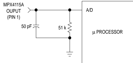
Figure 3. Decoupling Filter for Sensor to Microprocessor Interface
