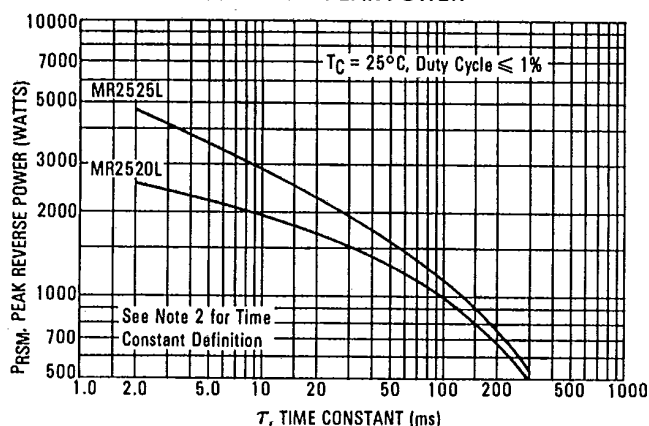
FIGURE 2 — PEAK POWER
