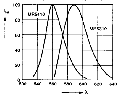
Relative Spectral Emission I rel = f(λ)
