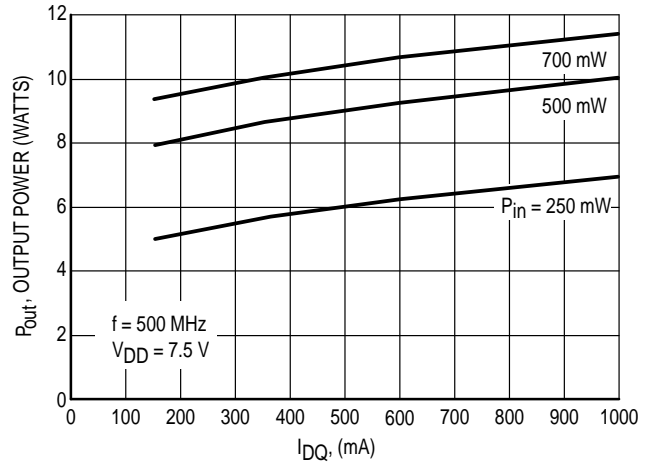
Figure 11. P_{out} versus I_{DQ}
