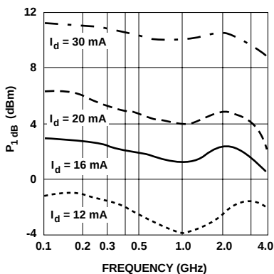
Figure 4. Output Power at 1 dB Gain
