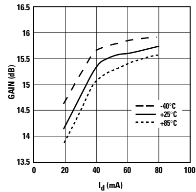
Figure 6. Gain vs. I_d and Temperature at 2 GHz.
