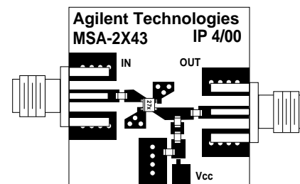
Figure 6. Complete 1.9 GHz Amplifier.
