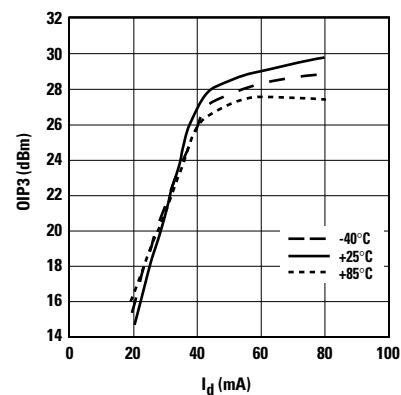
Figure 9. OIP3 vs. I_d and Temperature at 2 GHz.
