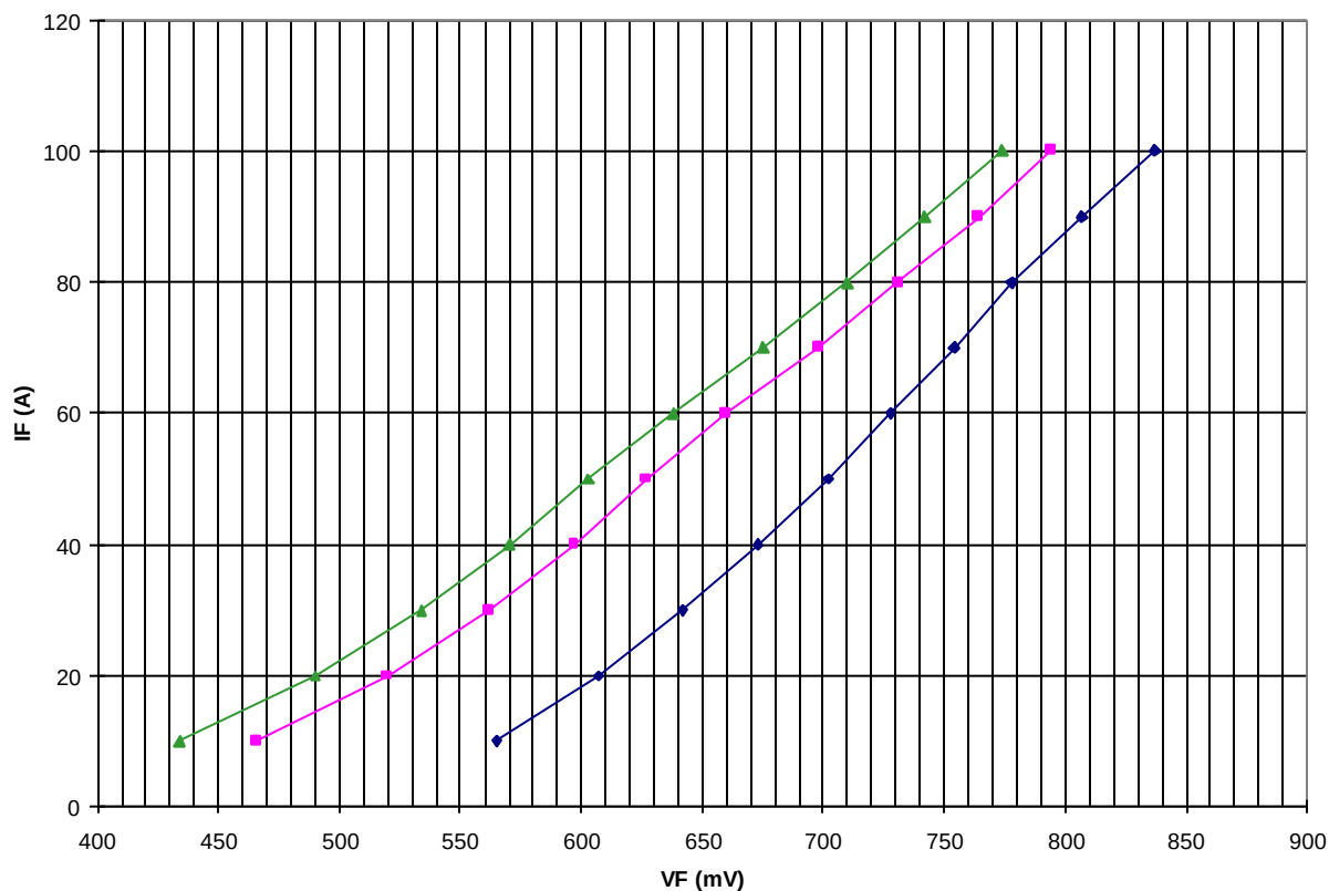
VF vs IF Typical Curves
