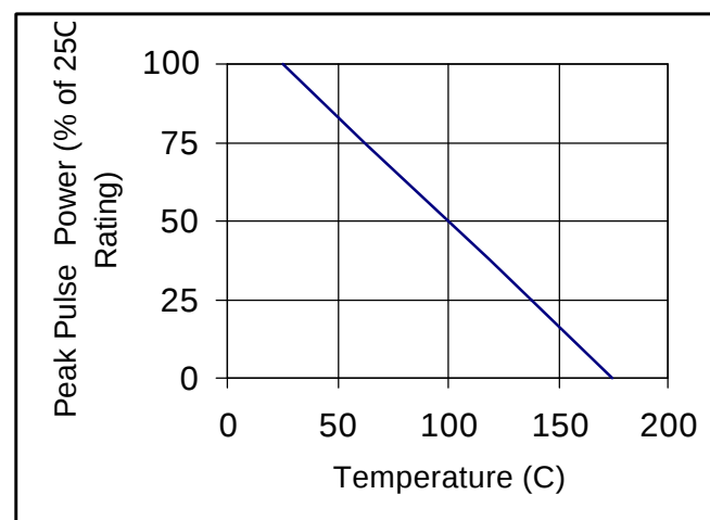
Fig.2 Derating Curve
