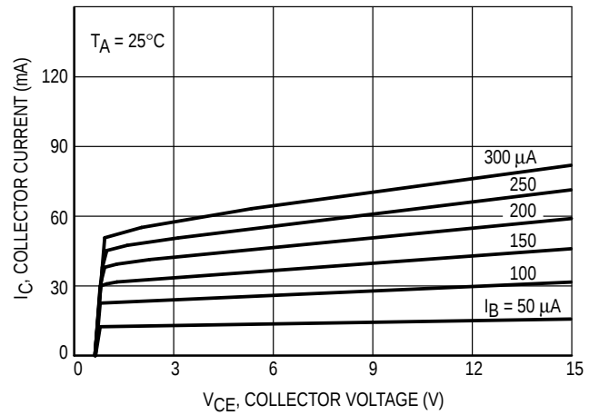
Figure 2. I_C - V_{CE}
