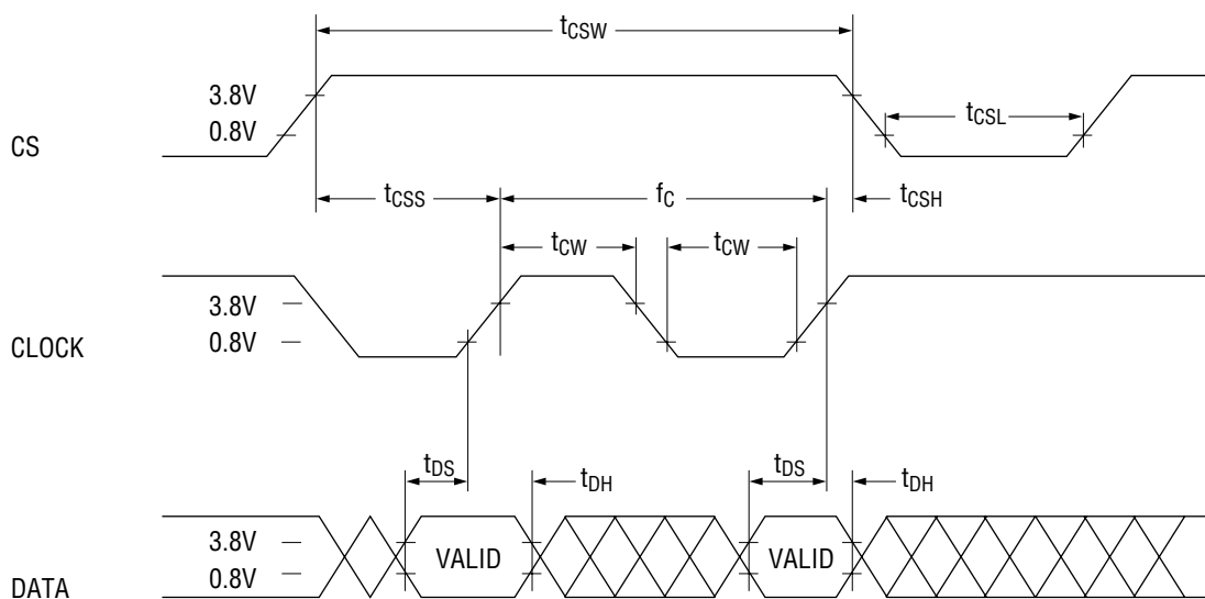
Fig. 1 Data Input Timing
