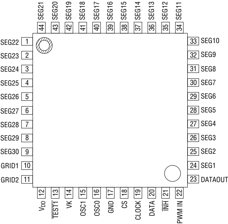
44-Pin Plastic Package
