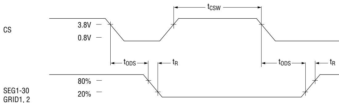
Fig. 4 SEG &amp; GRID Driver Output Timing
