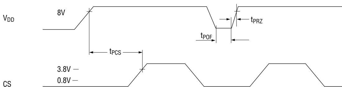
Fig. 3 Power-On Timing
