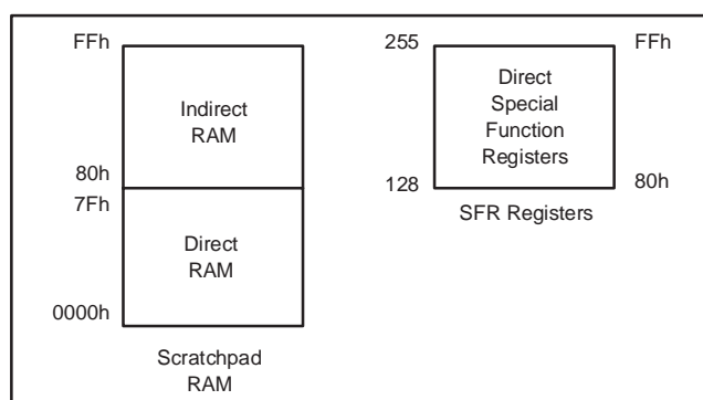
Figure 19. Register Map
