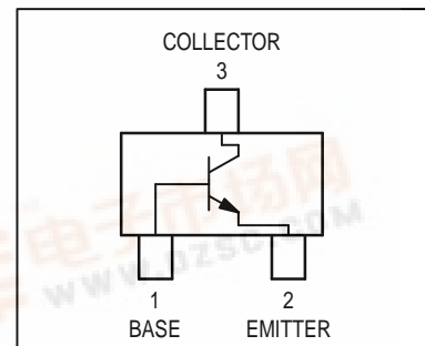
CASE 419-02, STYLE 3 SC-70/SOT-323
