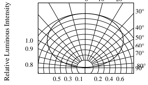
FIG.6 RADIATION DIAGRAM
