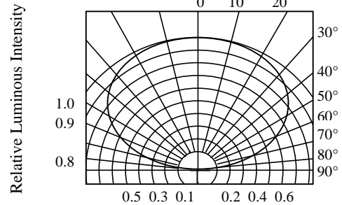
FIG.6 RADIATION DIAGRAM
