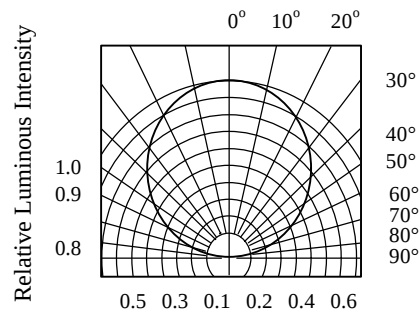
FIG.6 RADIATION DIAGRAM
