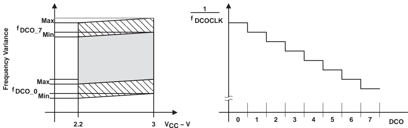
Figure 12. DCO Characteristics
