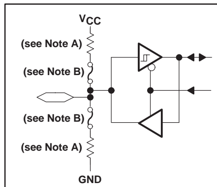
I/O WITH SCHMITT-TRIGGER INPUT (P0.x, TP0.5)
