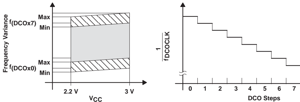
Figure 4. DCO Characteristics
