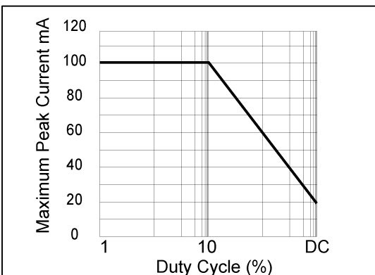
Maximum Peak Current vs Duty Cycle
