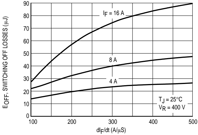
Figure 12. Typical Switching Off Losses
