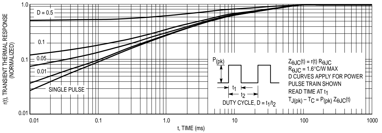
Figure 14. Thermal Response
