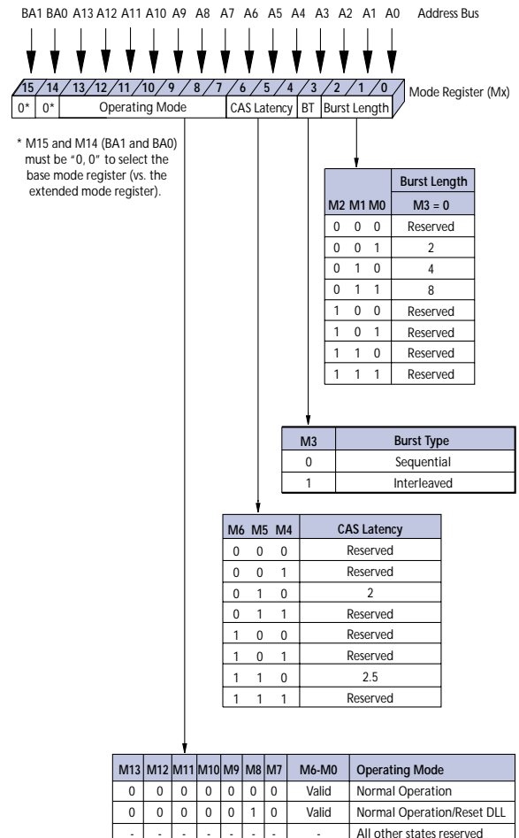
Figure 5: Mode Register Definition
