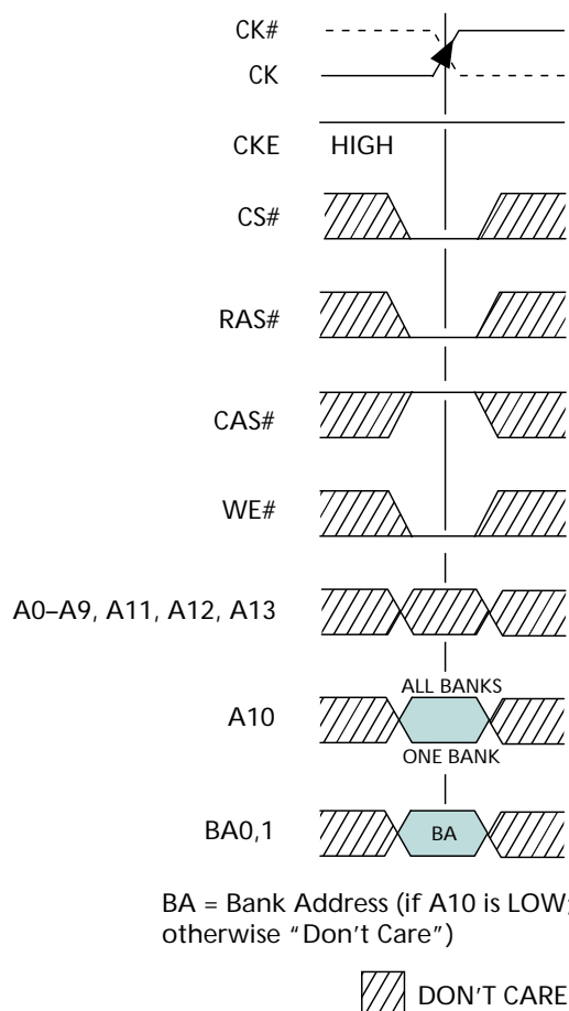
Figure 29: PRECHARGE Command
