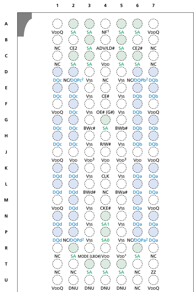
TOP VIEW
