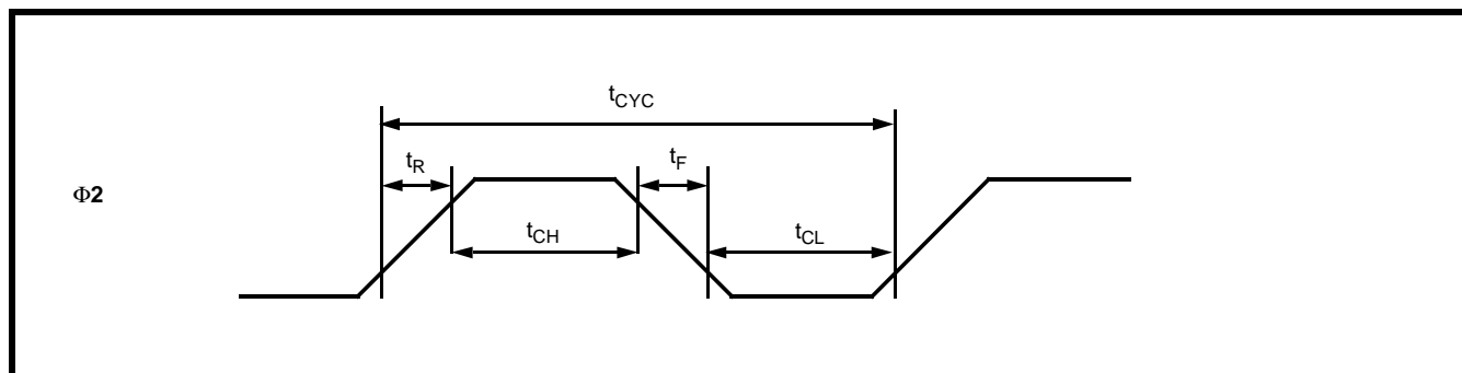
Figure 17 - \Phi 2 Pulse
