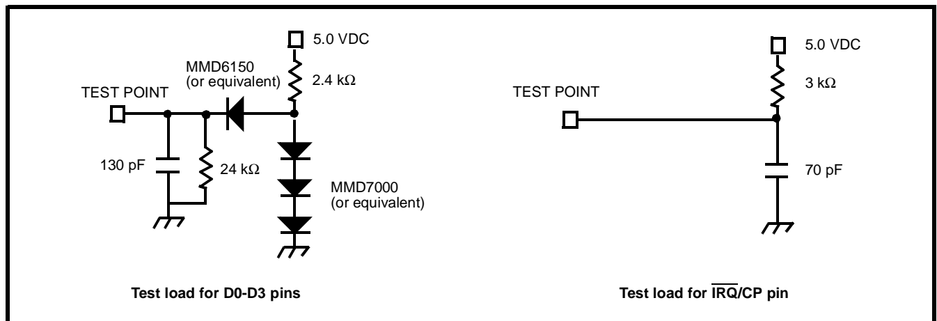
Figure 14 - Test Circuit
