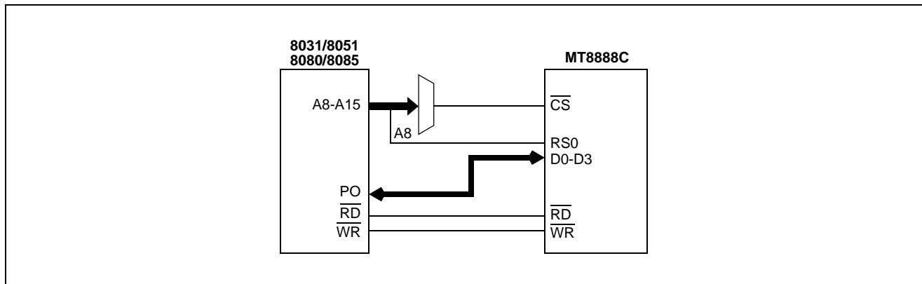
Figure 14 - MT8888C Interface Connections for Various Intel Micros
