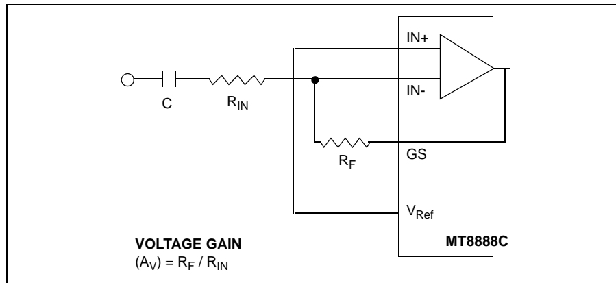
Figure 3 - Single-Ended Input Configuration
