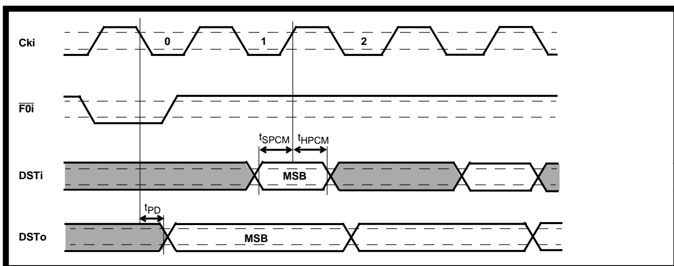
Figure 6 - PCM Timing
