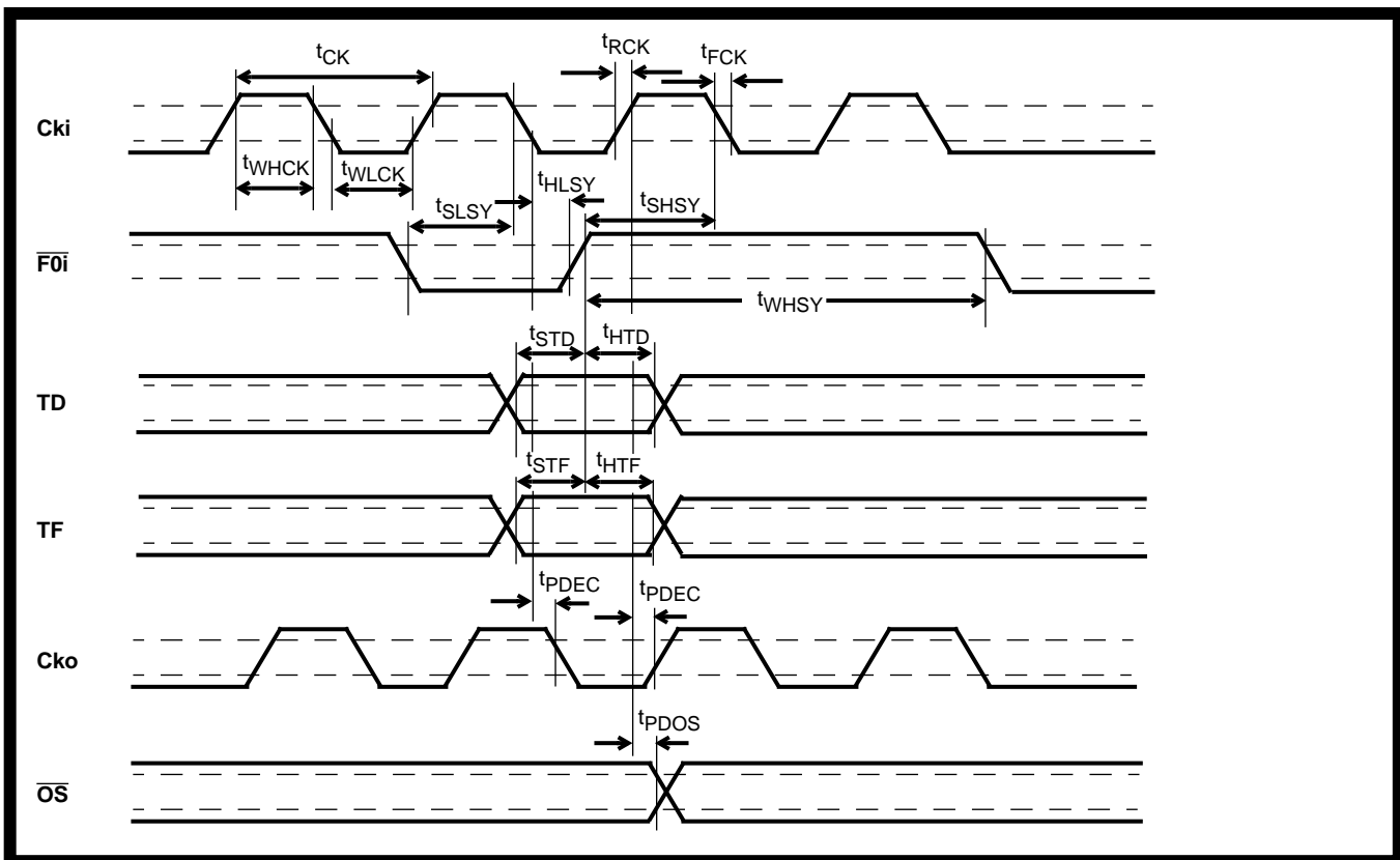
Figure 5 - Clock Timing
