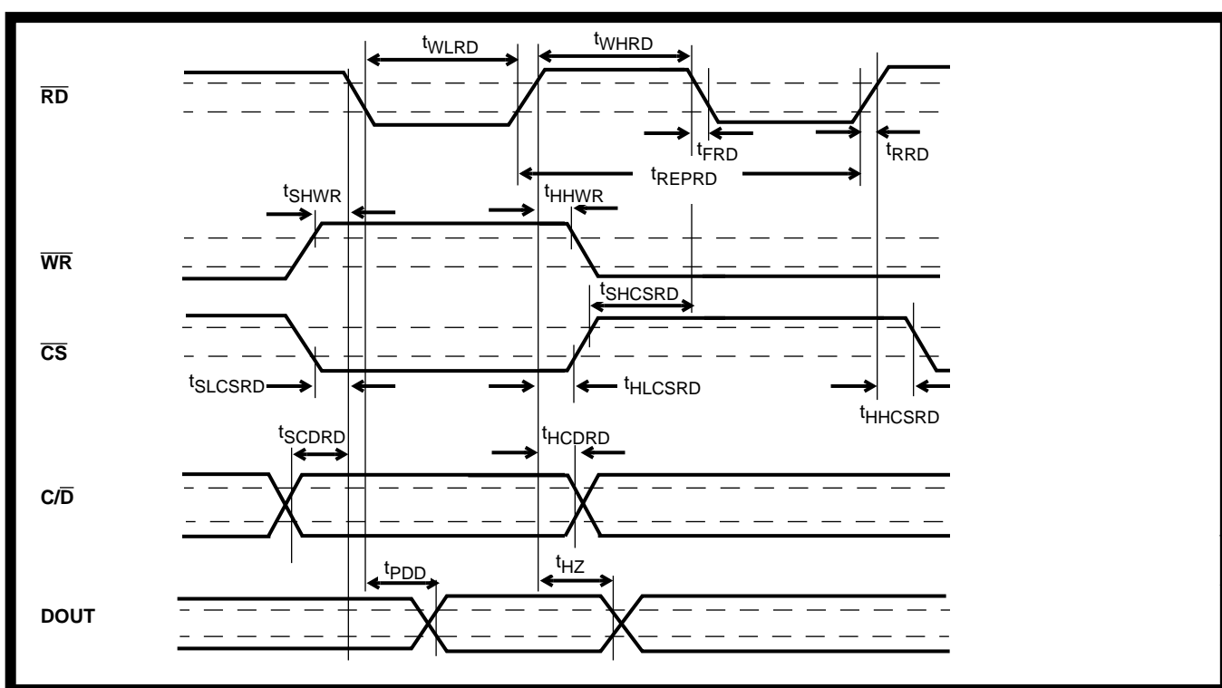
Figure 9 - Read Timing Characteristics
