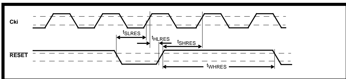
Figure 7 - Reset Timing
