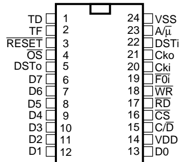
Figure 2 - Pin Connections
