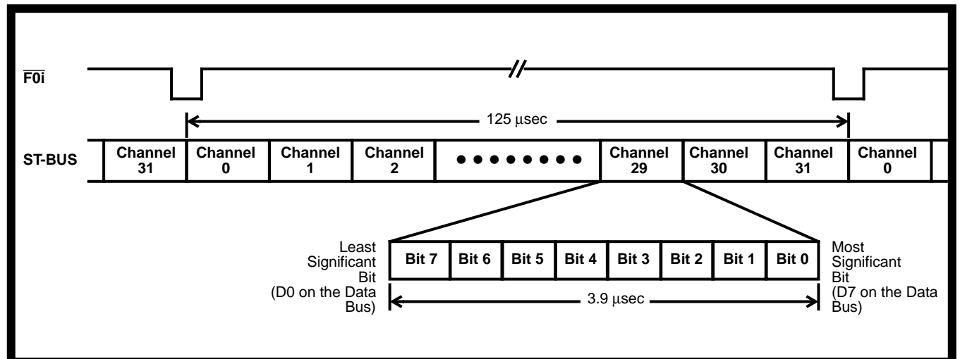
Figure 24 - ST-BUS Format
