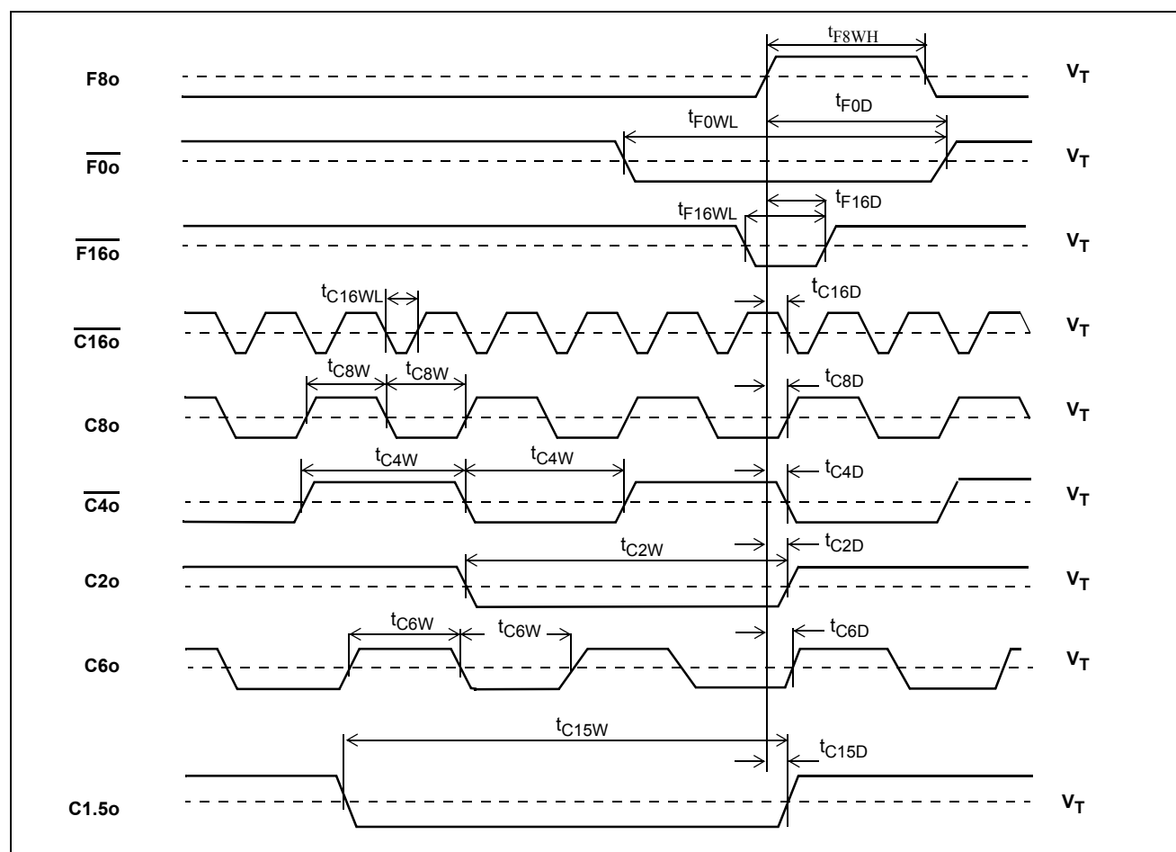
Figure 18 - Output Timing 1
