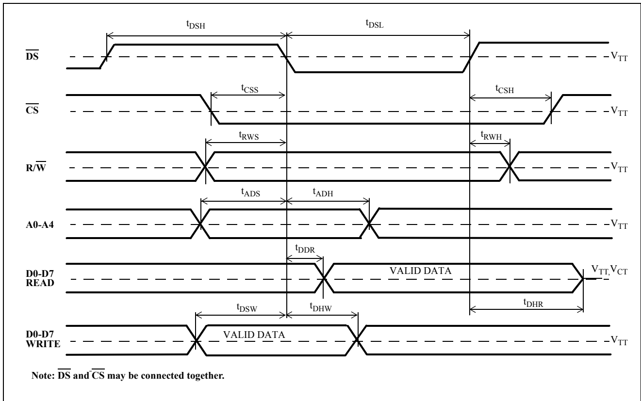
Figure 15 - Microport Timing
