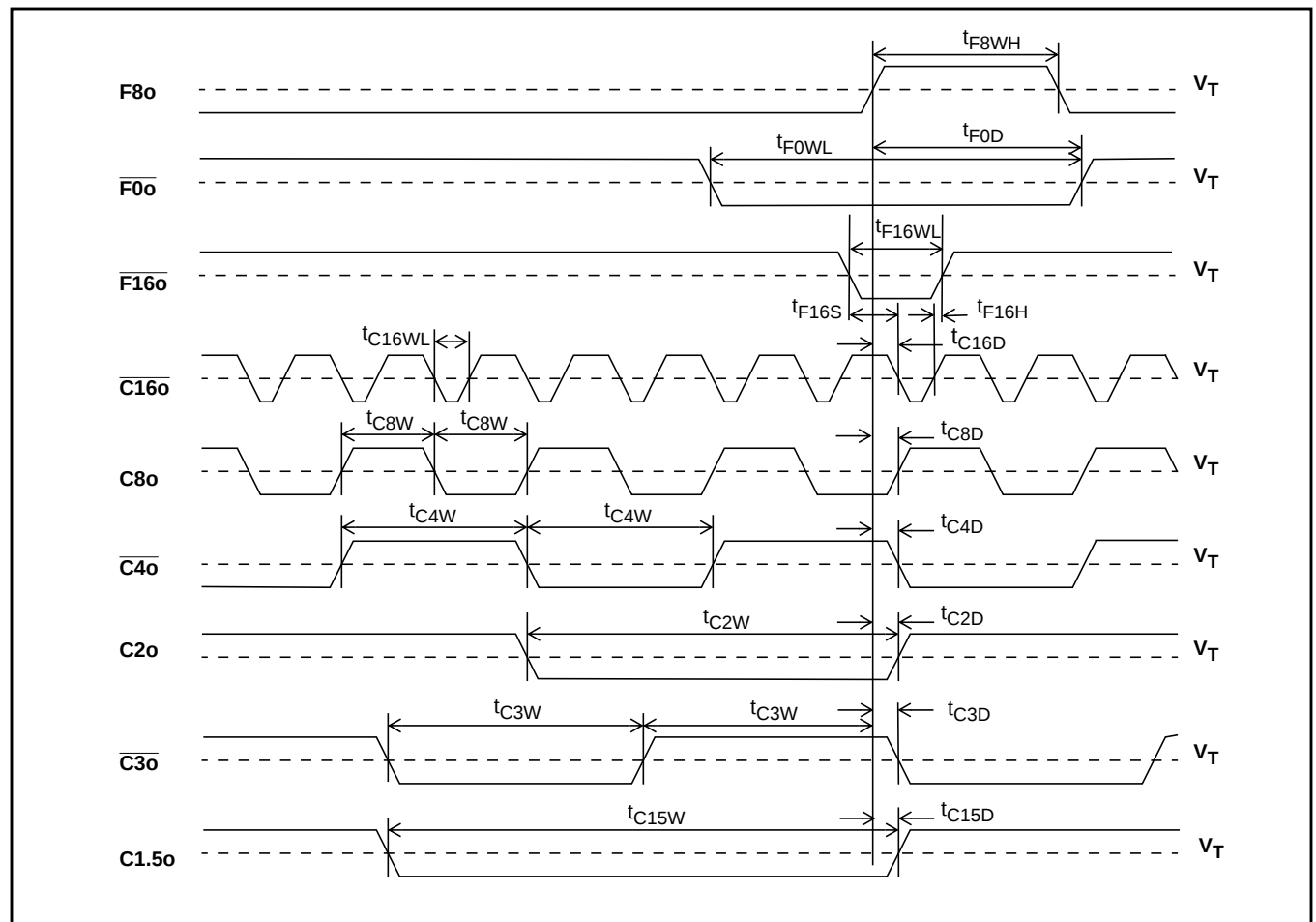
Figure 20 - Output Timing 1
