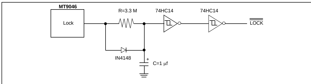
Figure 11 - Time-constant Circuit
